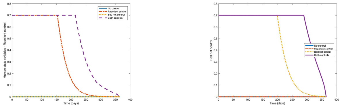
Figure 2: Control variables, u_1 and u_2 , for the multiple strategies
