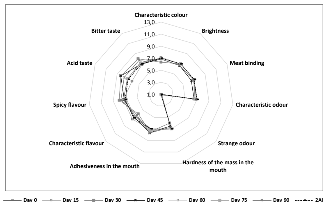
Figure 2. Sensory profile of "Alheira" during storage at 4 °C in an intensity scale of the main descriptors considered in a QDA for 2AIP with dried L. plantarum ST153Ch. 2AIC: control without starter culture.
